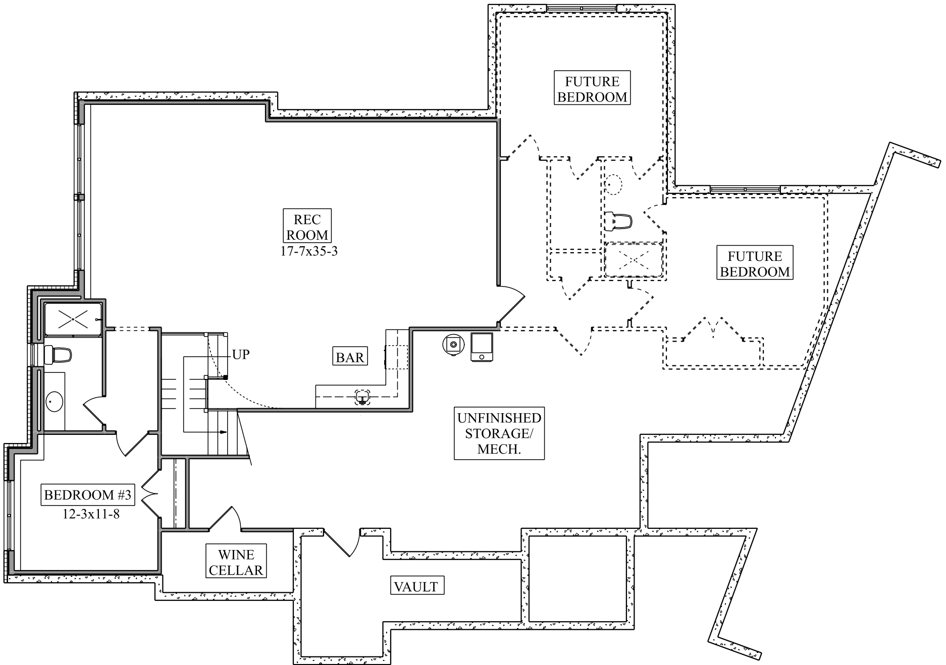
LOWER FLOOR PLAN 1,185 FinSqFt
