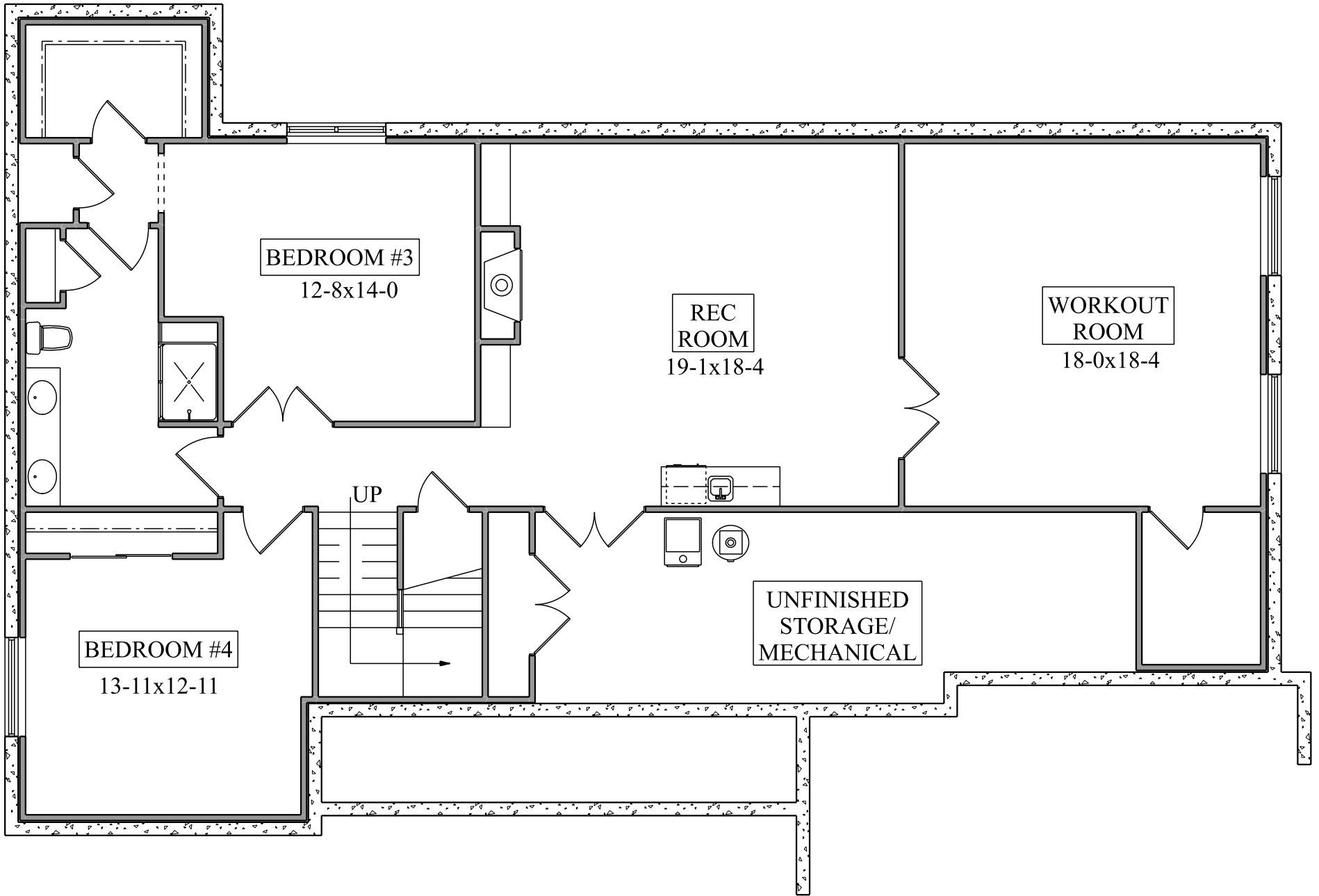
LOWER FLOOR PLAN 1,688 FinSqFt
