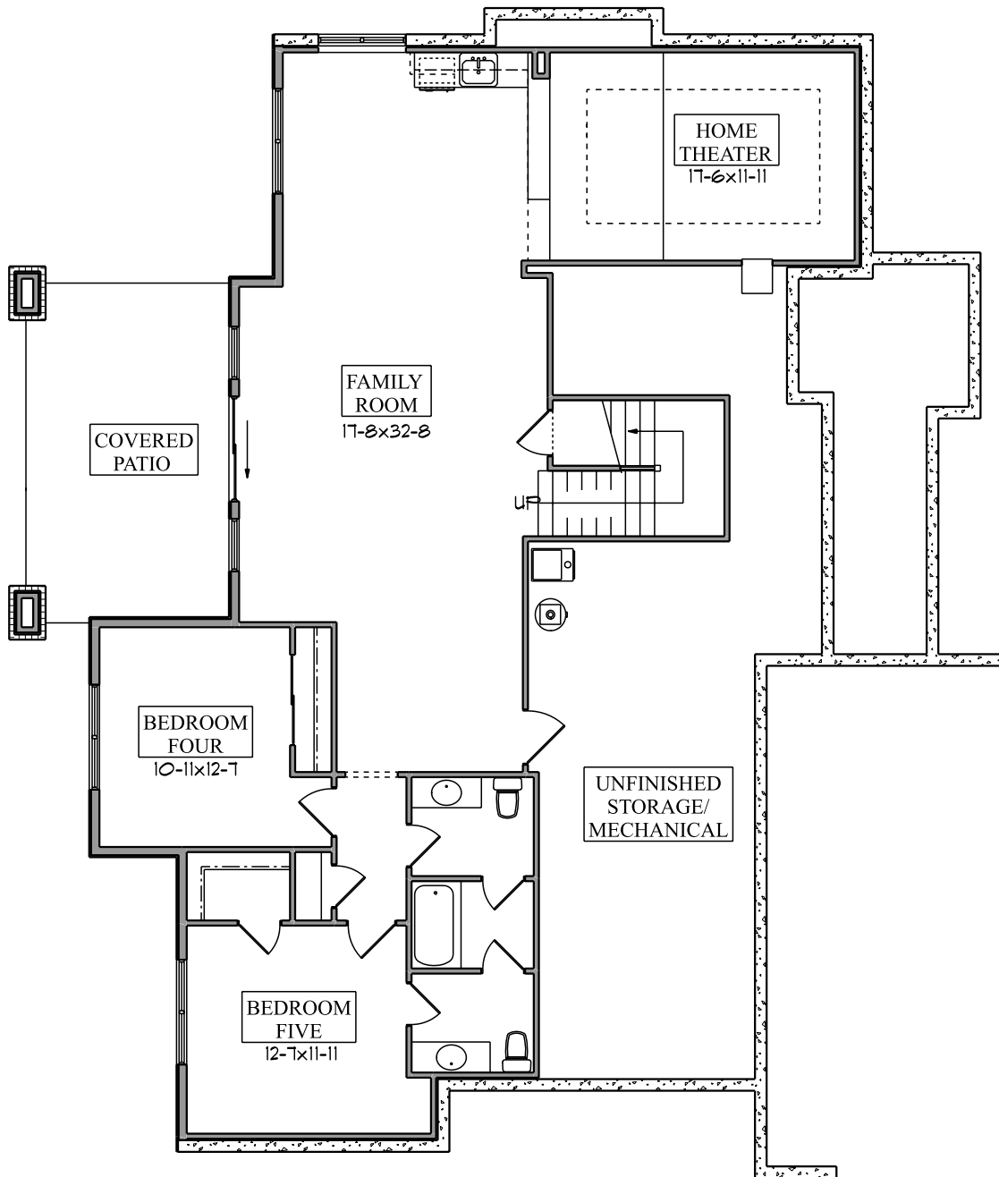
LOWER FLOOR PLAN 1,495 FinSqFt
