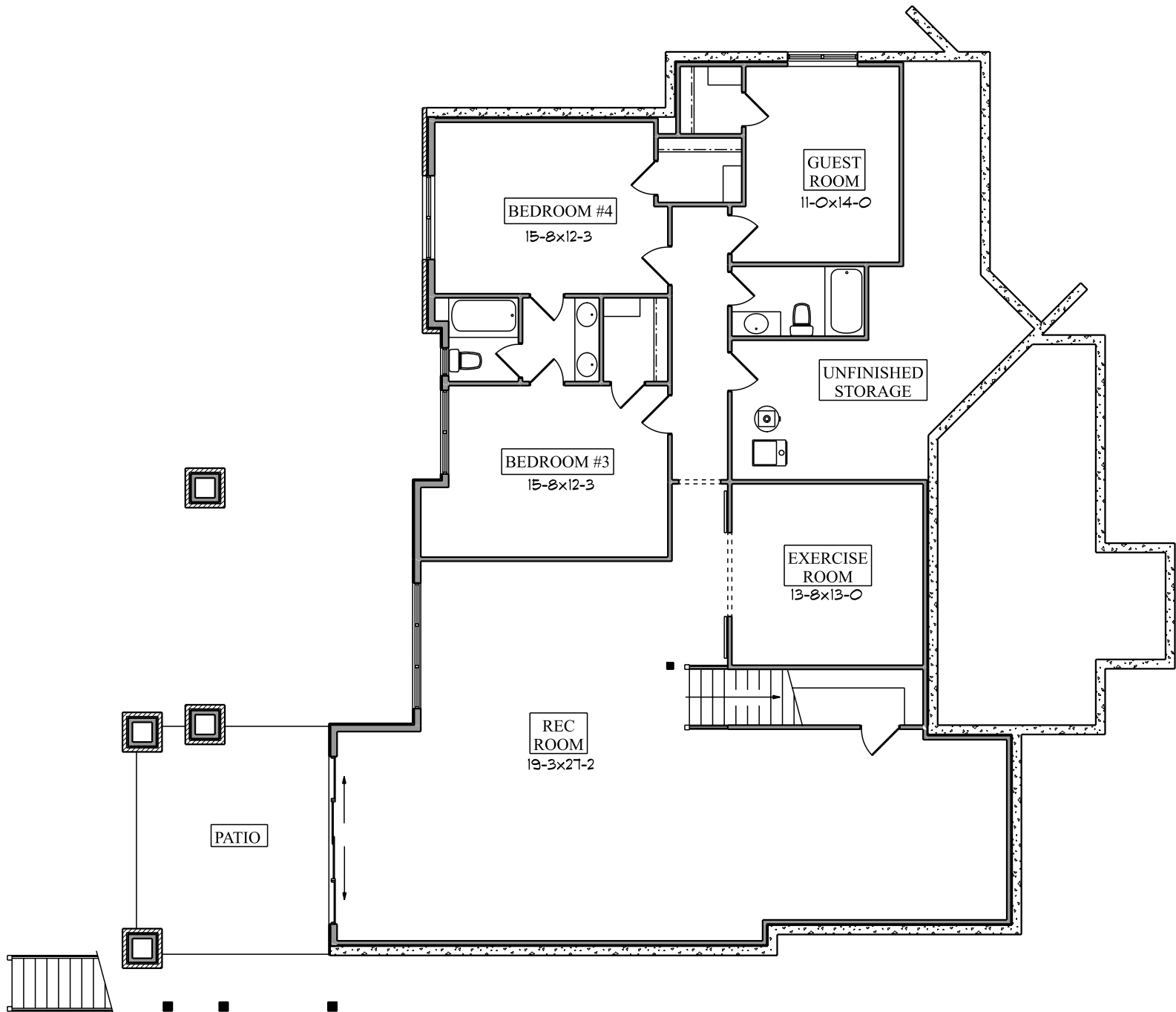
LOWER FLOOR PLAN 2,279 FinSqFt
