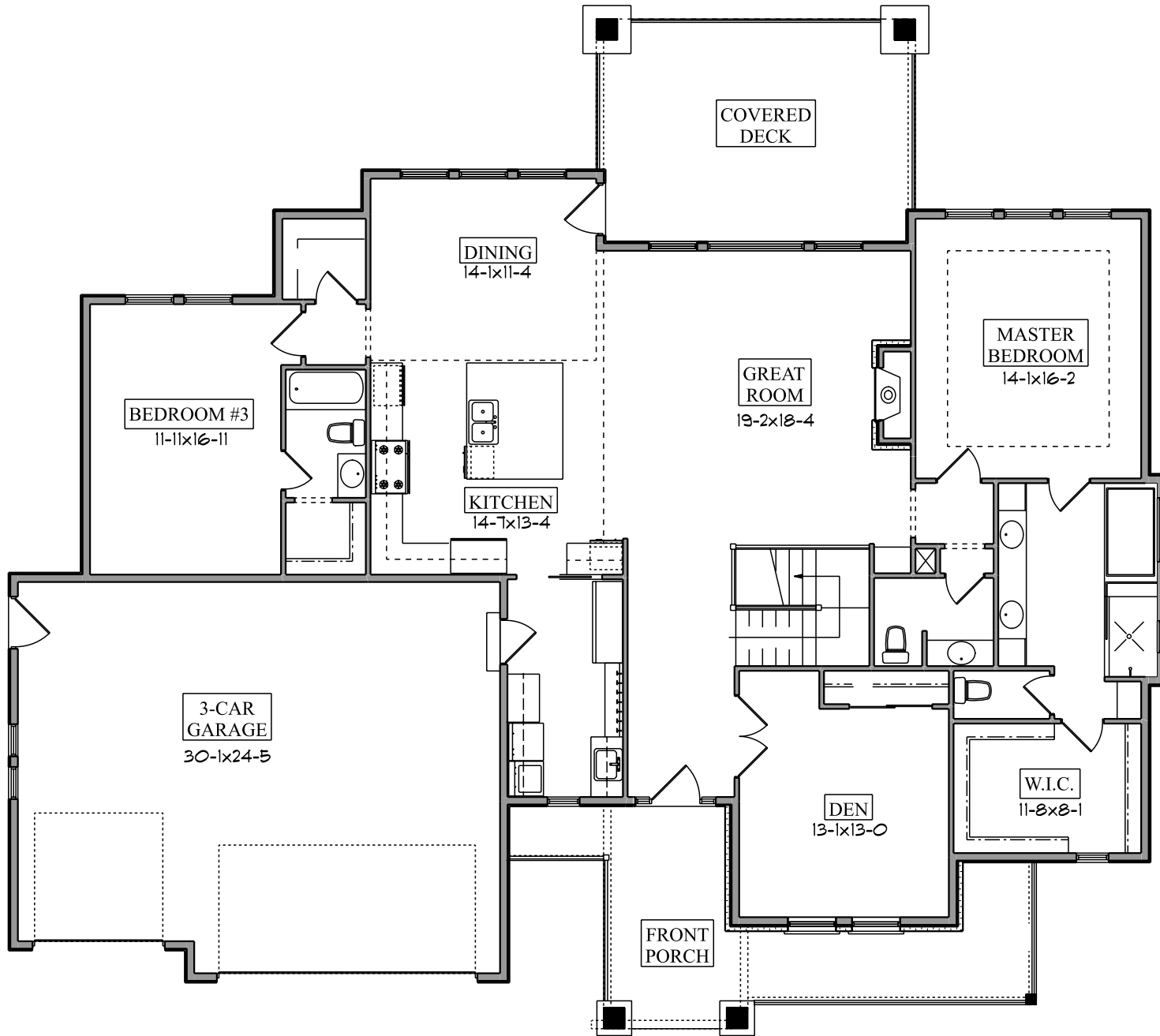
MAIN FLOOR PLAN 2,194 FinSqFt
