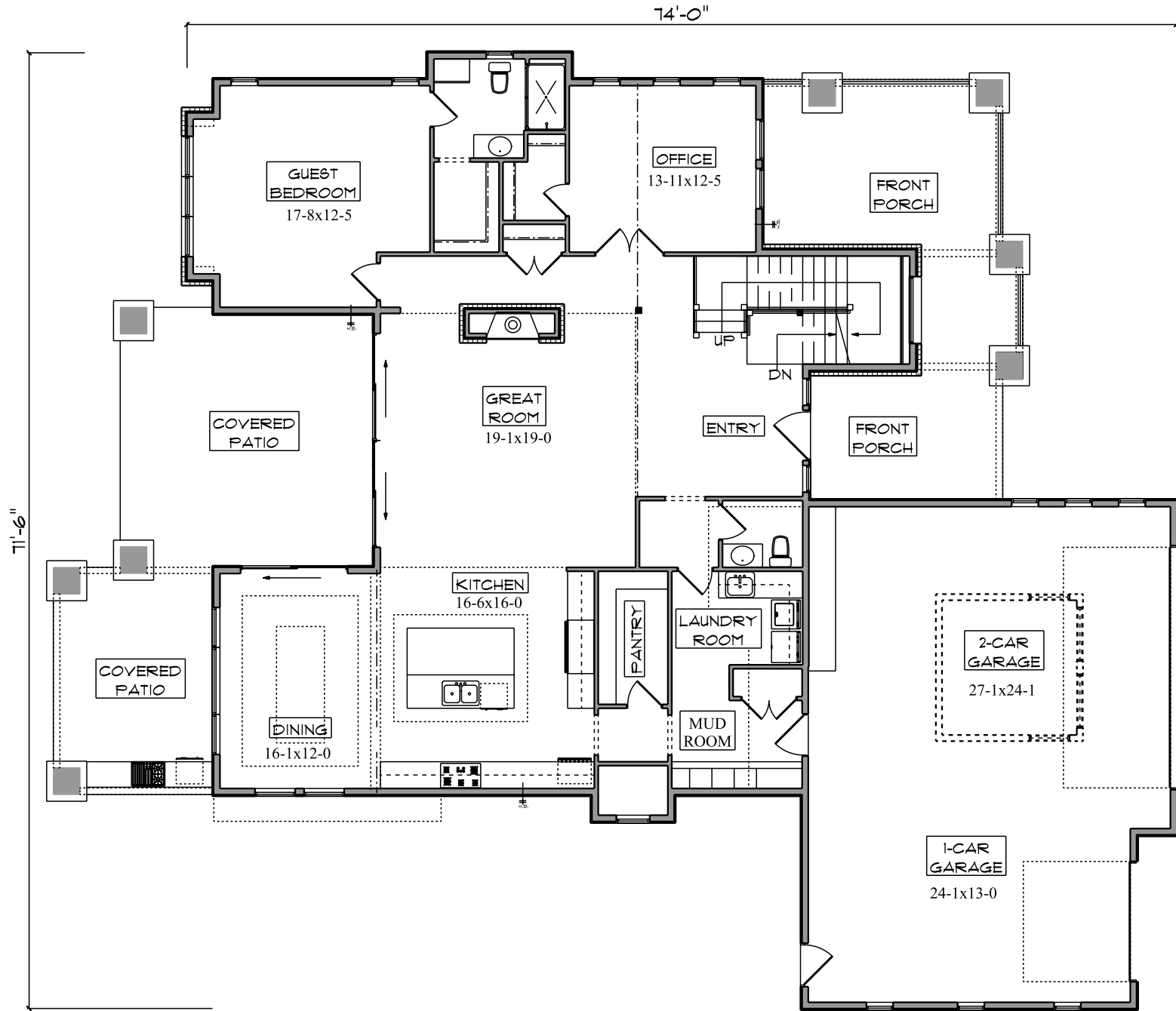
MAIN FLOOR PLAN 2,236 FinSqFt
